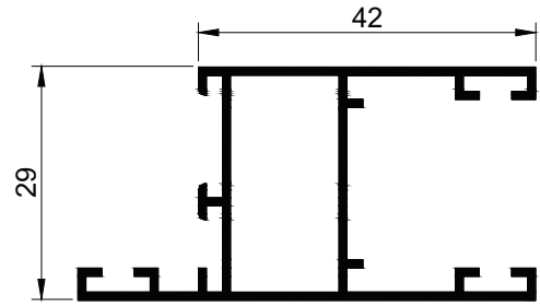
3021 m = 0,680 \text{ kg/m}
