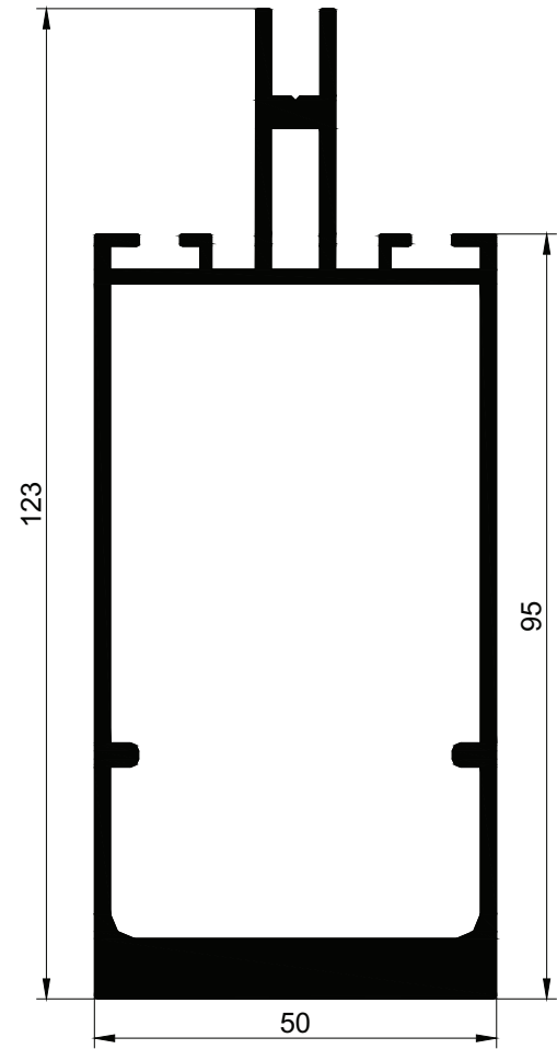
2062 m = 2,745 kg/m
