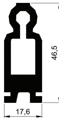
3418 m = 1,136 \text{ kg/m}
