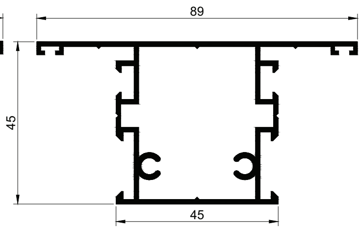
3422 m = 1,174 \text{ kg/m}
