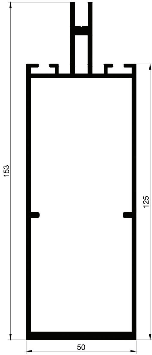
2061 m = 2,572 kg/m
