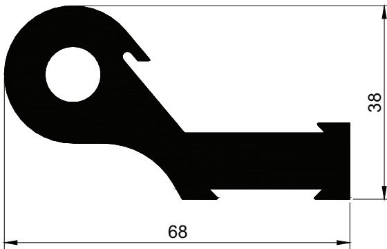
6026 m = 2,749 kg/m
