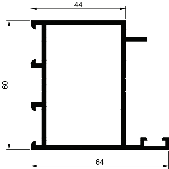
6001 m = 1,351 \text{ kg/m}
