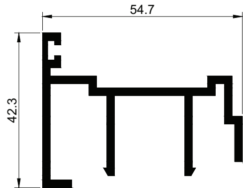
6012 m = 1,014 \text{ kg/m}
