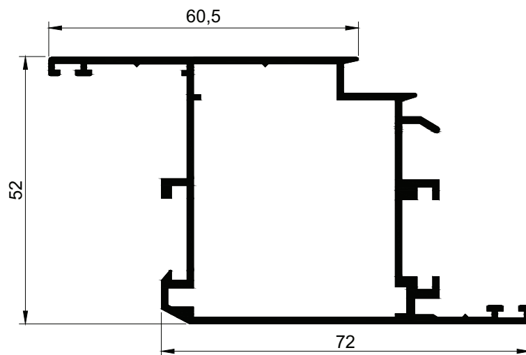
3698 m = 1,110 kg/m
