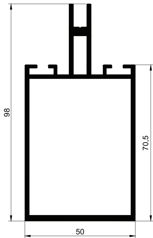
2063 m = 1,801 kg/m
