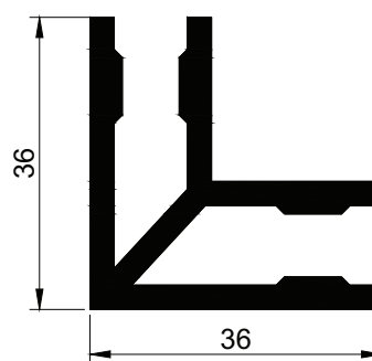
3066B m = 1,093 \text{ kg/m}
