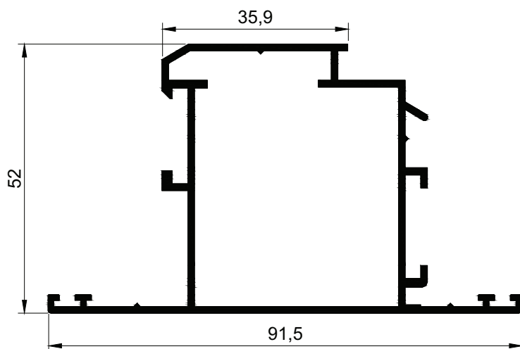
3421 m = 1,089 kg/m
