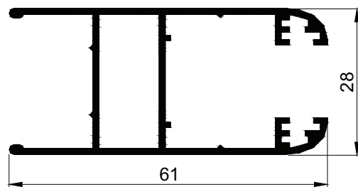
3371 m = 0,690 \text{ kg/m}
