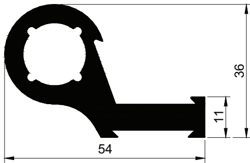
6024 m = 1,674 kg/m
