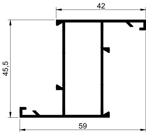
3079 m = 0,656 kg/m
