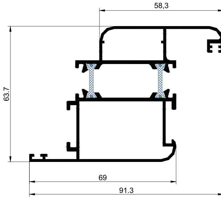
3467 m = 1,523 kg/m
