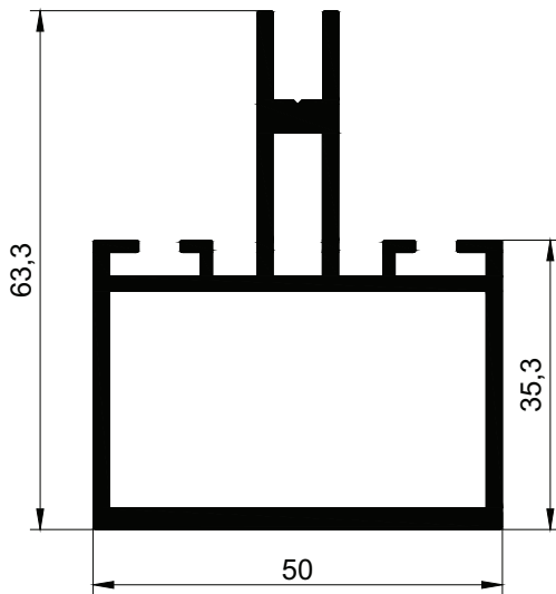
2064 m = 1,426 kg/m
