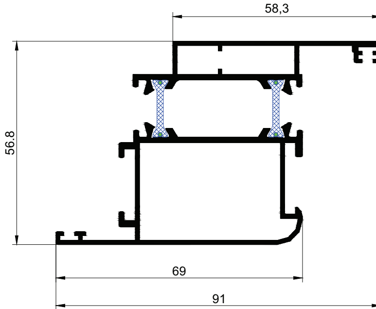
3469 m = 1,456 kg/m
