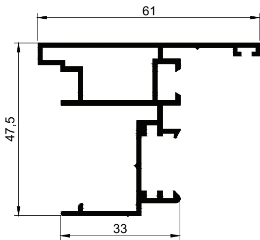
3552 m = 0,830 \text{ kg/m}
