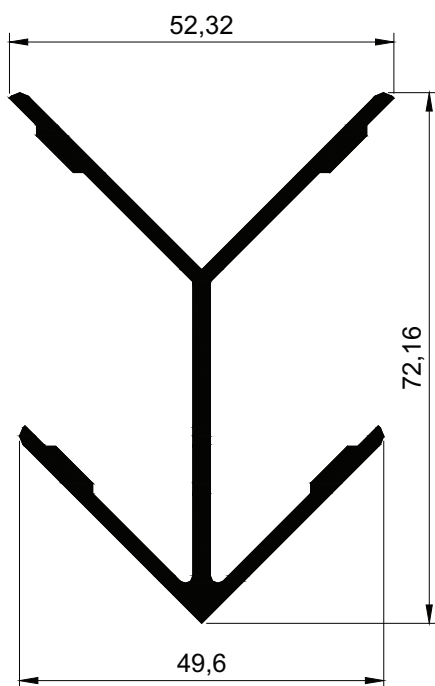
3066A m = 1,169 \text{ kg/m}
